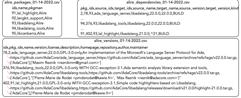
(b) Excerpts from Alire ecosystem data in CSV serialization syntax.
